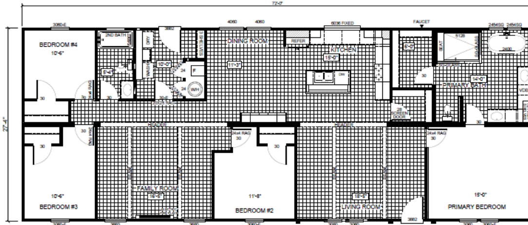
SHOWN WITH OPTIONAL FRONT ELEVATION
